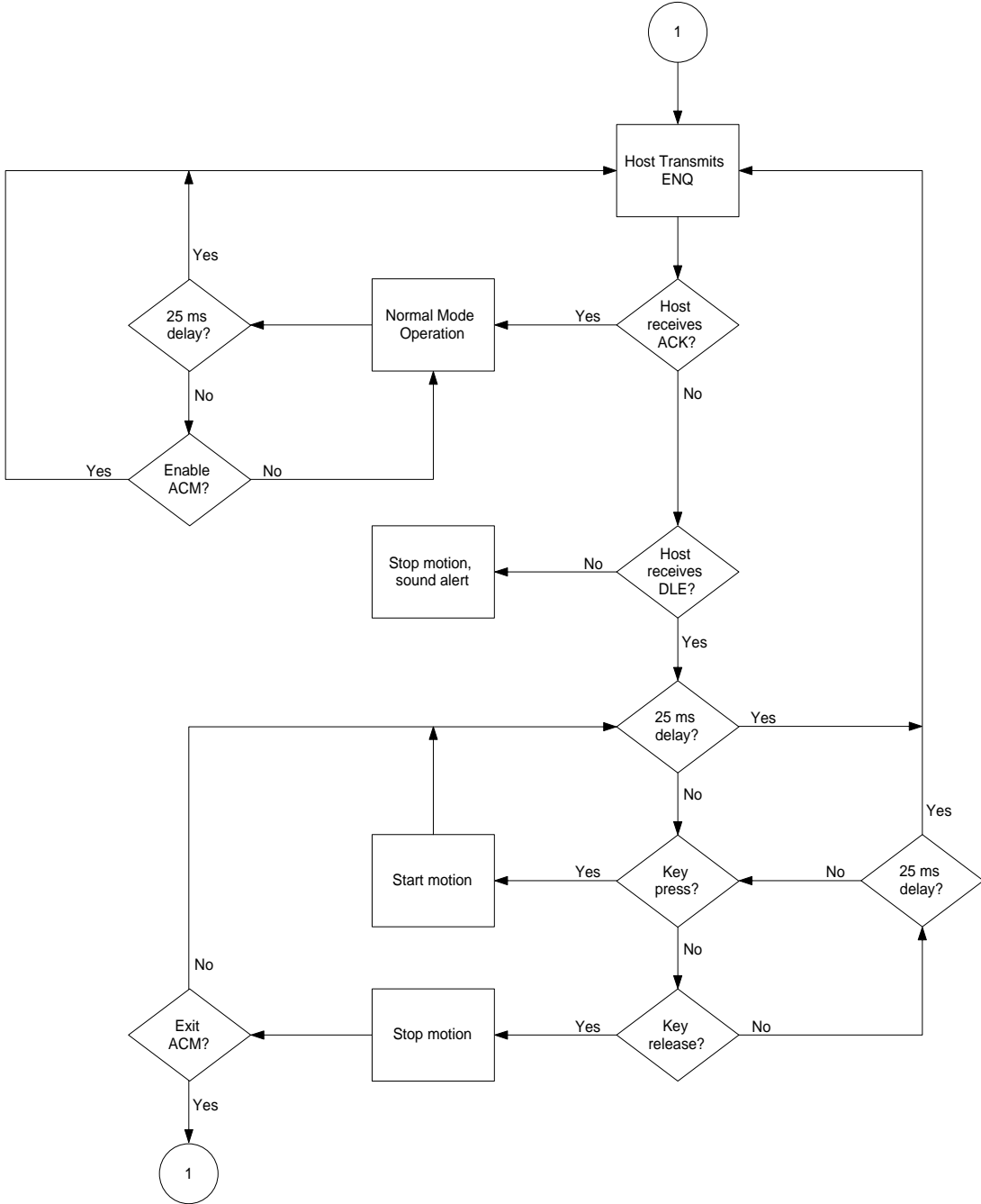
Figure 5-3: Using ACM in a Robotic Environment Flowchart
