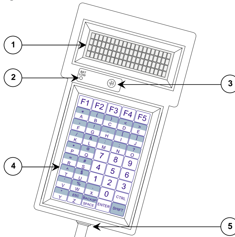
Figure 2-1: 80 Series Controls and Indicators
