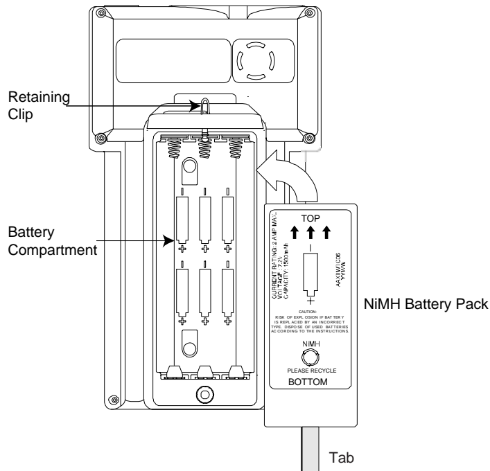
Figure 2-7: Changing Batteries
