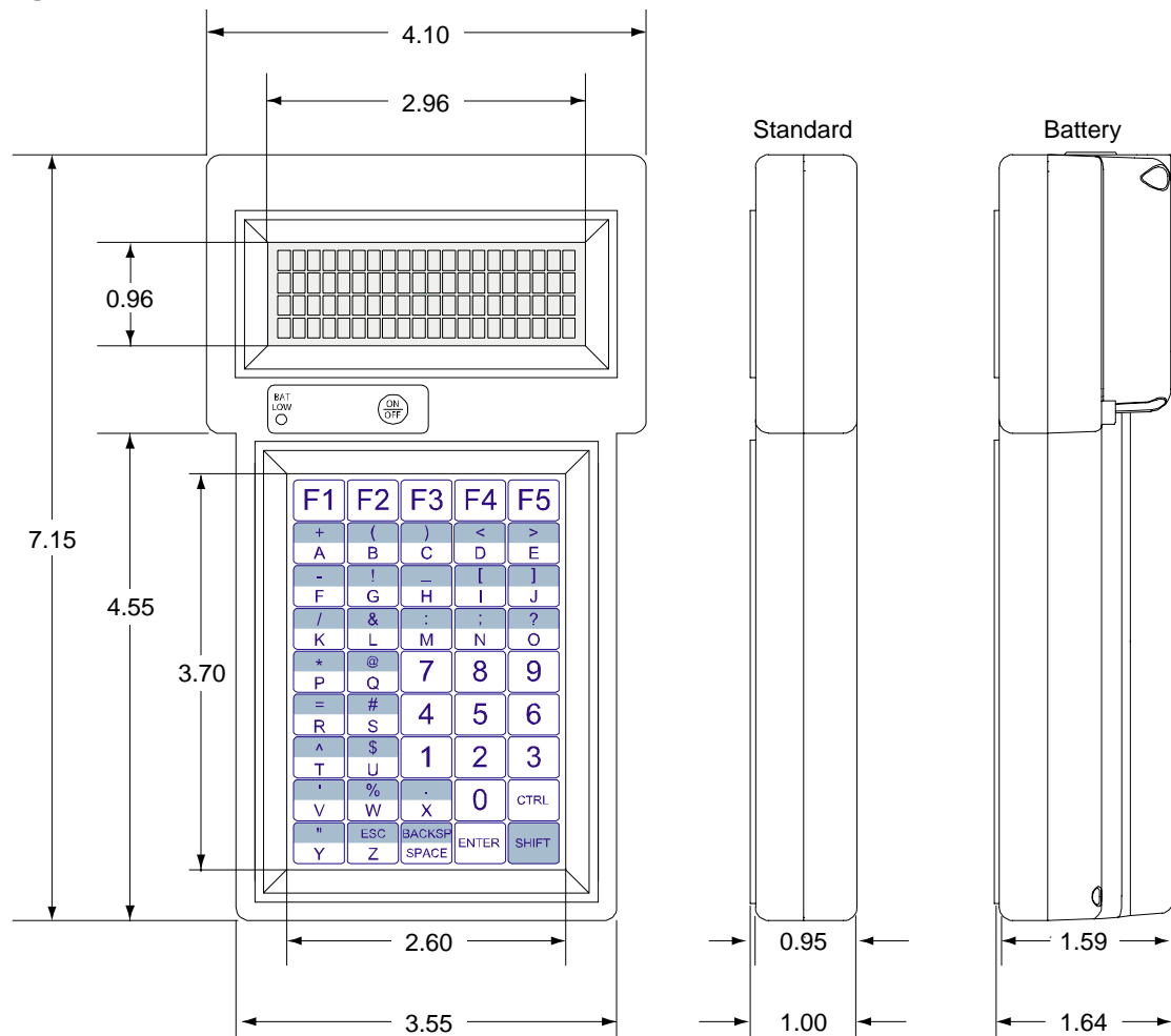
Figure A-1: 80 Series Terminal Case Dimensions
