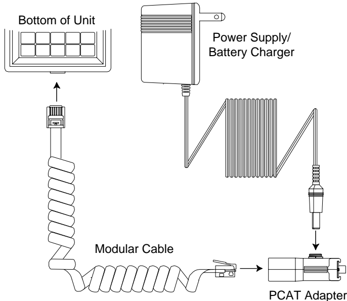
Figure 2-5: Cable Connections
