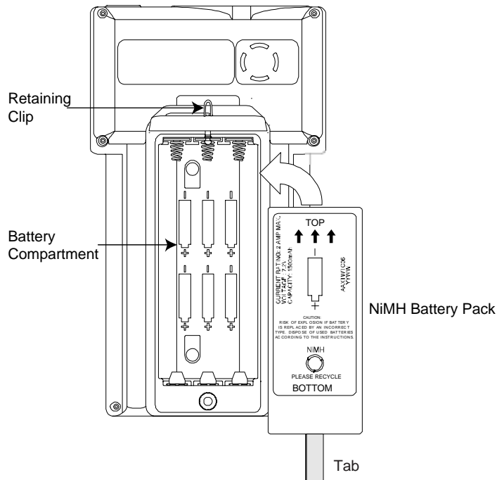
Figure 2-6: Battery Orientation
